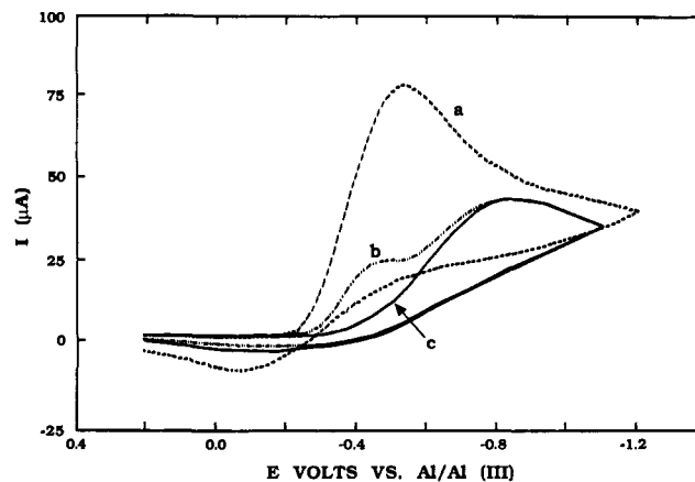
Figure 4. Cathodic staircase cyclic voltammetry for the 0.8:1 melt as MAC is added to the melt initially 53 mM in DMA and 107 mM in \text{ImHCl}_2 ; [\text{MAC}] = 13.7 (a), 49.8 (b), 75 mM (c). Other conditions as in Figure 1.
