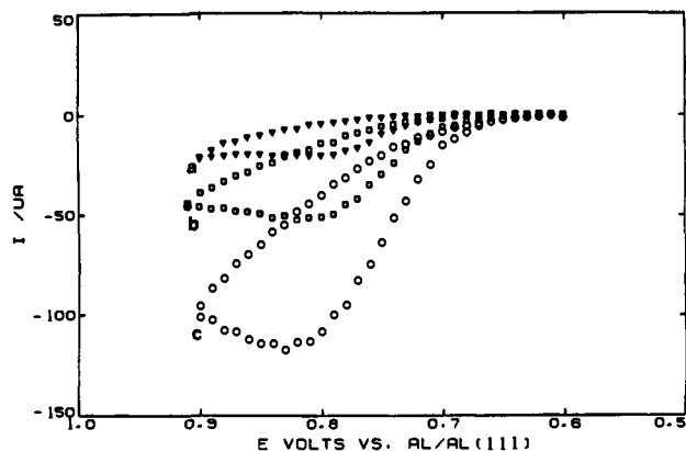
Figure 1. Staircase cyclic voltammogram for DMA in the 0.8:1 melt at a Pt electrode, A = 2 \times 10^{-2} \text{ cm}^2 ; scan rate 250 \text{ mV s}^{-1} (step height 10 mV, step width 40 ms); [\text{DMA}] = 10.4 (a), 29.7 (b), 52.8 mM (c).
