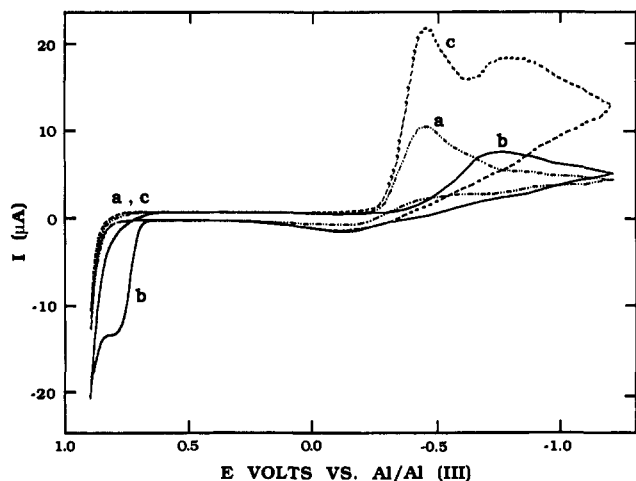
Figure 3. Staircase cyclic voltammograms for DMA in the 0.8:1 melt: (a) melt background; (b) 17 mM DMA added; (c) as in b, but 30 mM \text{ImHCl}_2 added. Conditions as in Figure 1. Sweep rate 100\text{ mV s}^{-1} (step height 10 mV, step width 100 ms).
